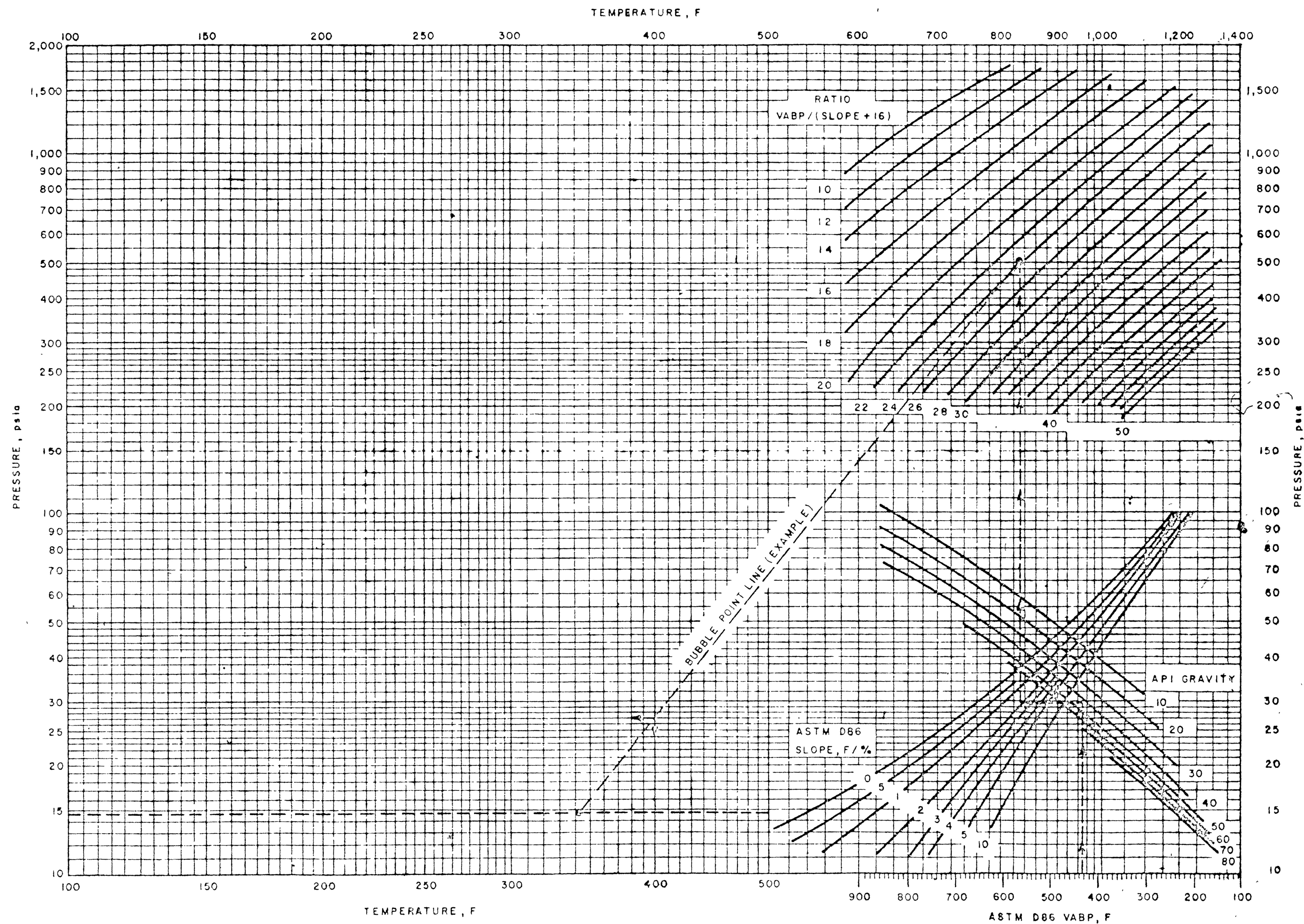
FIGURE 3 - ASTM D86 Distillation Temperature and Equalization Flash Vaporization Temperature Pressure Conversion Chart.
